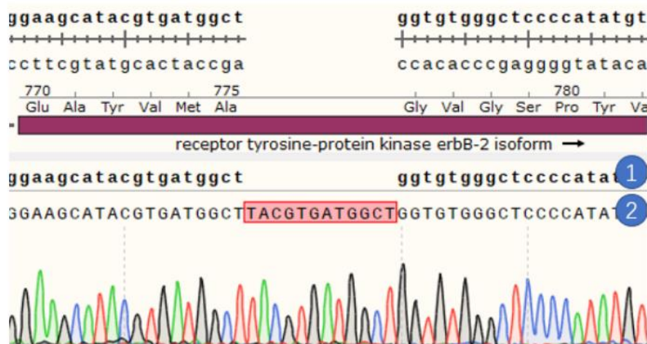
Figure 1 | The ERBB2 mutation analysis by Sanger sequencing.(1 represents the wild-type sequence, and 2 represents the sequence after knock-in mutation.)
